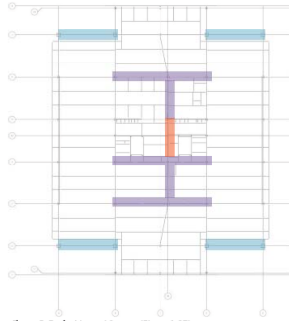
Figure 5: Typical Lateral System (Floors 1-27)
