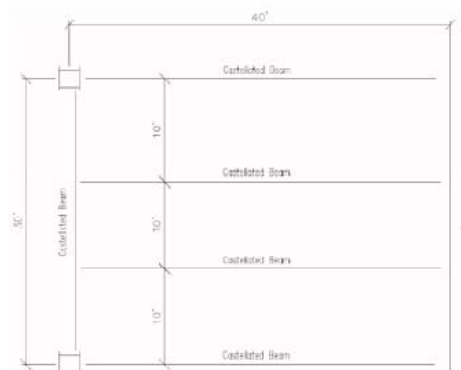
Figure15: Castelled Beam w/ Typical Metal Decking Alternative
