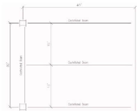
Figure14: Castelled Beam w/ Long Span Metal Decking Alternative
